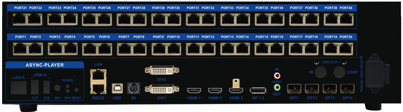
M40 rear-panel interface map. The asynchronous-player bay and Genlock are configuration-dependent.
