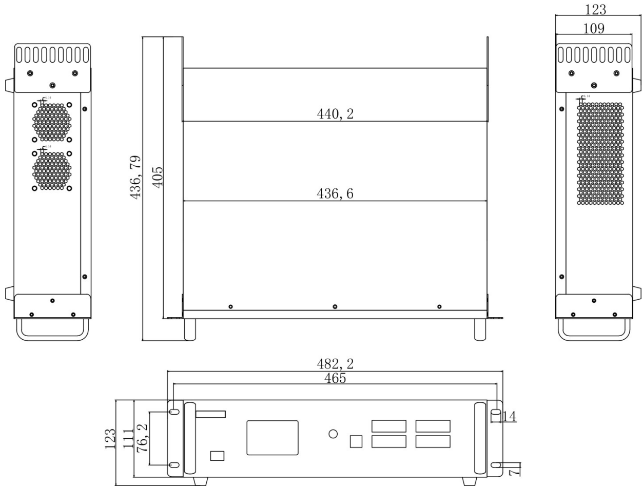
Mechanical dimensions. Units: mm. Drawing tolerance: +/-0.3 mm.
