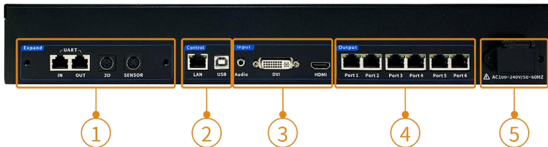
Rear Panel
