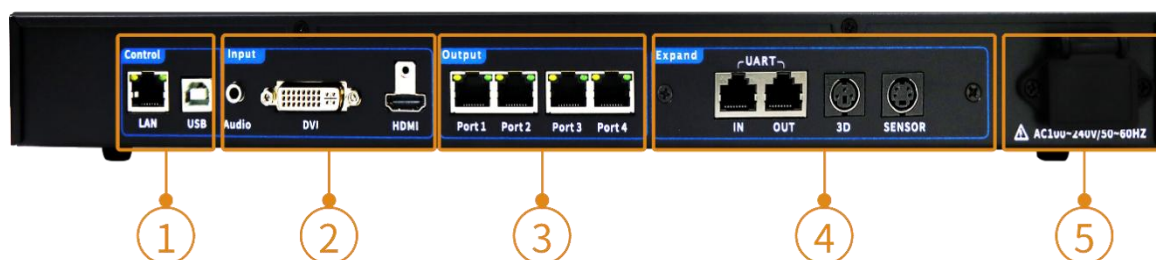
Rear Panel
