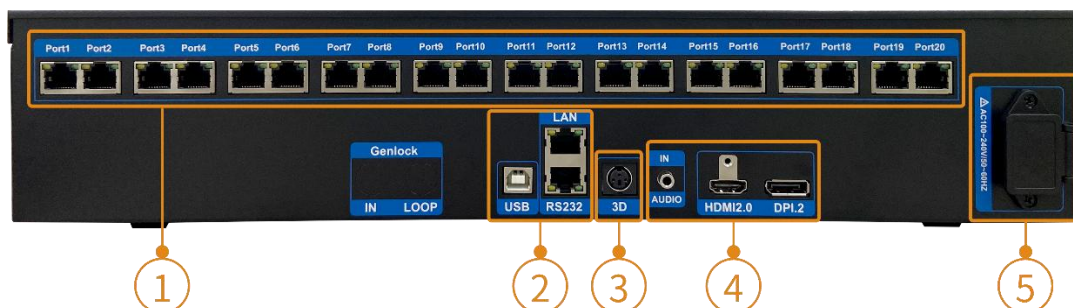
Rear Panel
