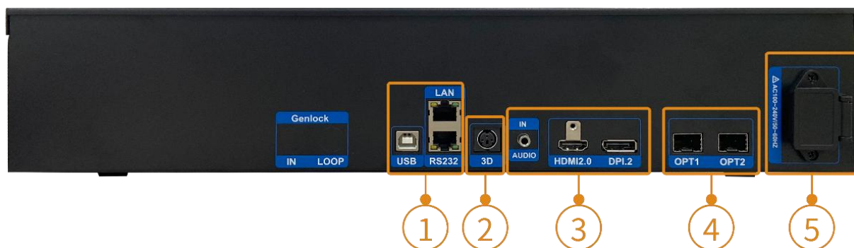
Rear Panel
